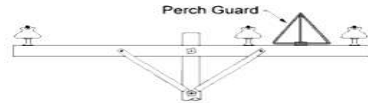
Figure 7.62. Drawing of a perch guard between insulators.
