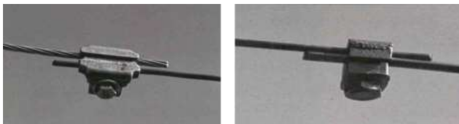
Figure 7.60. LM connector.
