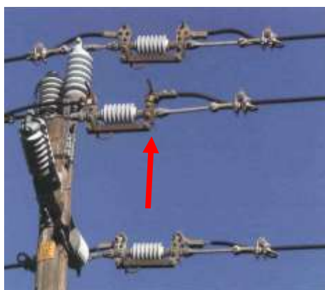
Figure 7.55. Inline disconnect.
