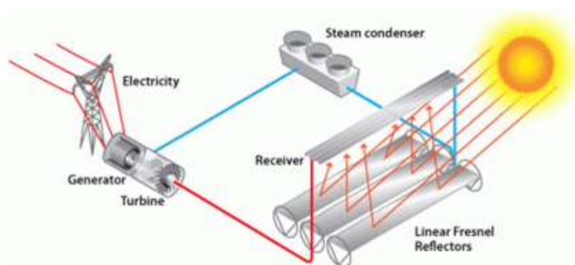
Figure 7.70. Linear power systems with linear Fresnel reflectors.
