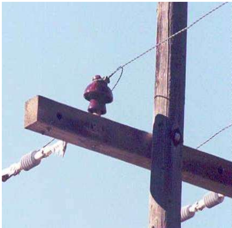
Figure 7.52. Typical crossarm insulator on a wooden mounting peg.
