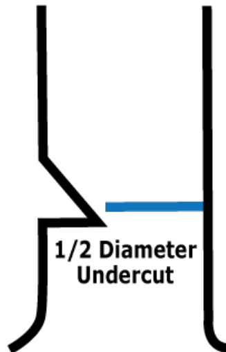
Figure: Candlestick with \frac{1}{2} diameter undercut.
